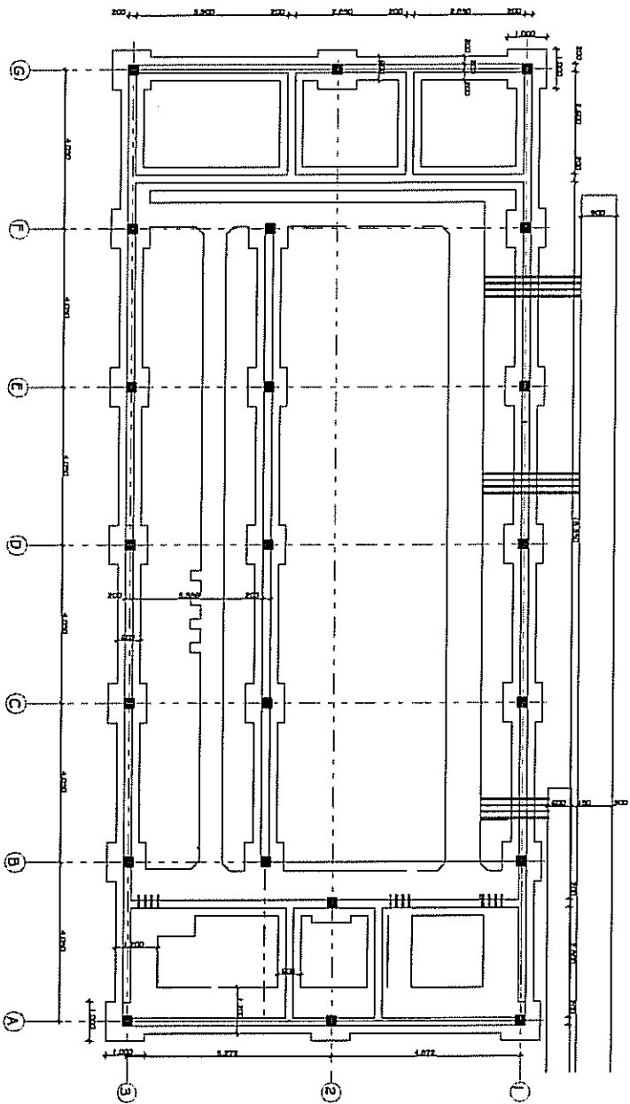
FOUNDATION FLOOR PLAN
